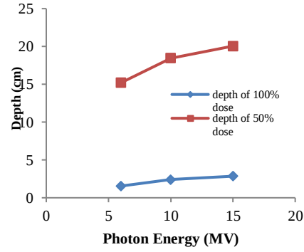
Figure 6: The fluctuation of depth of maximum dose and 50% dose with photon energy.
