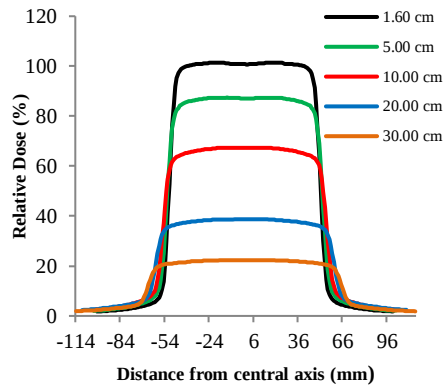
Figure 9: Profile doses curve for 6 MV photon beam at field size 10 x 10 cm 2 with various depth
