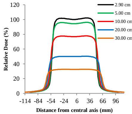
Figure 11: Profile doses curve for 15 MV photon beam at field size 10 x 10 cm 2 with various depth
