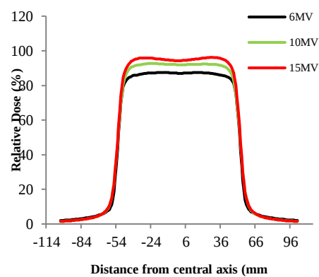
Figure 12: Profile doses curve for various photon beams at field size 10 x 10 cm 2 with 10 cm depth.
