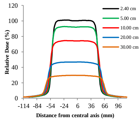
Figure 10: Profile doses curve for 10 MV photon beam at field size 10 x 10 cm 2 with various depth
