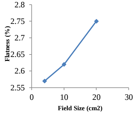
Figure 14: Variation of flatness with field sizes.
