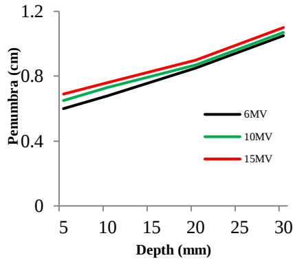
Figure 15: Variation of penumbra with depth for different photon beams with field size 10x10 cm 2
