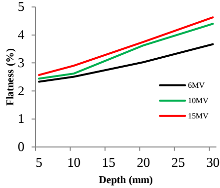
Figure 13: Variation of flatness with depth for different photon beams at field size 10x10 cm 2
