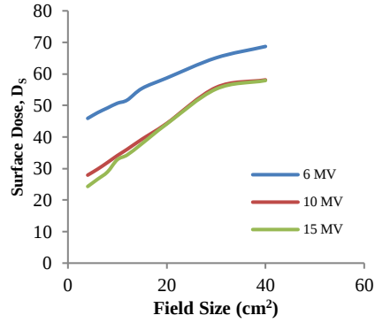
Figure 5: The fluctuation of surface dose for different field sizes.
